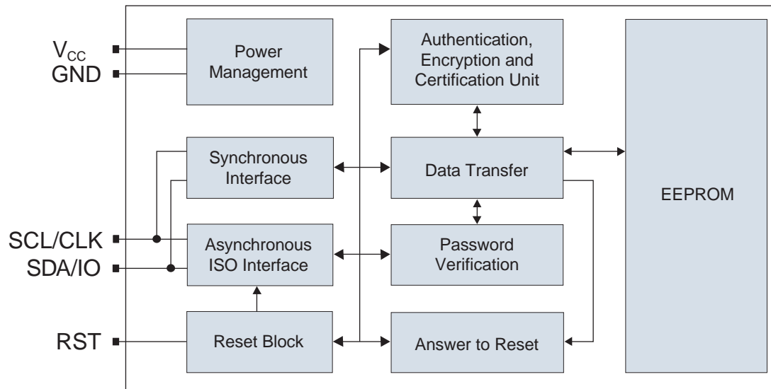
Figure 3-1. Block Diagram
