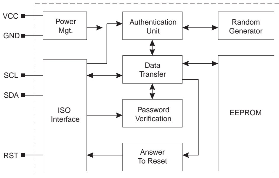
Figure 2-1. Block Diagram
