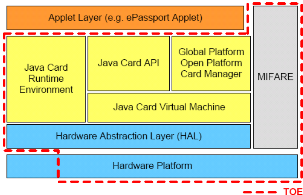
Figure 1: JCOP Architecture
