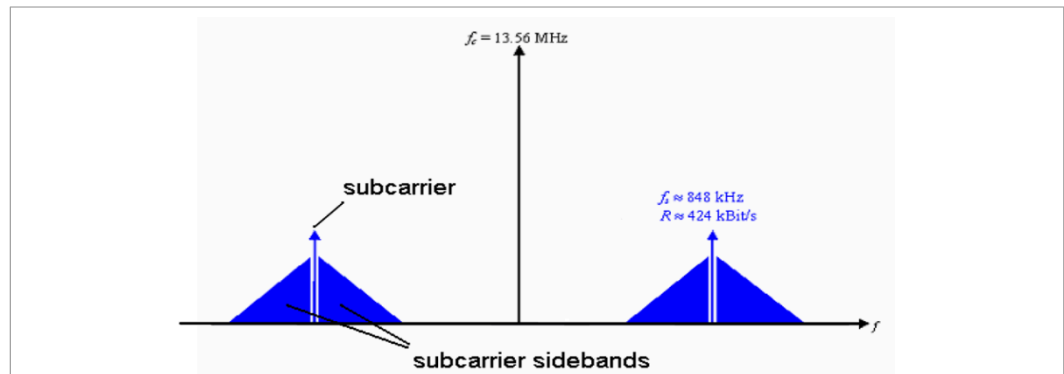
Figure 6. Theoretical needed PICC bandwidth for a data transfer at 424 kB/s
