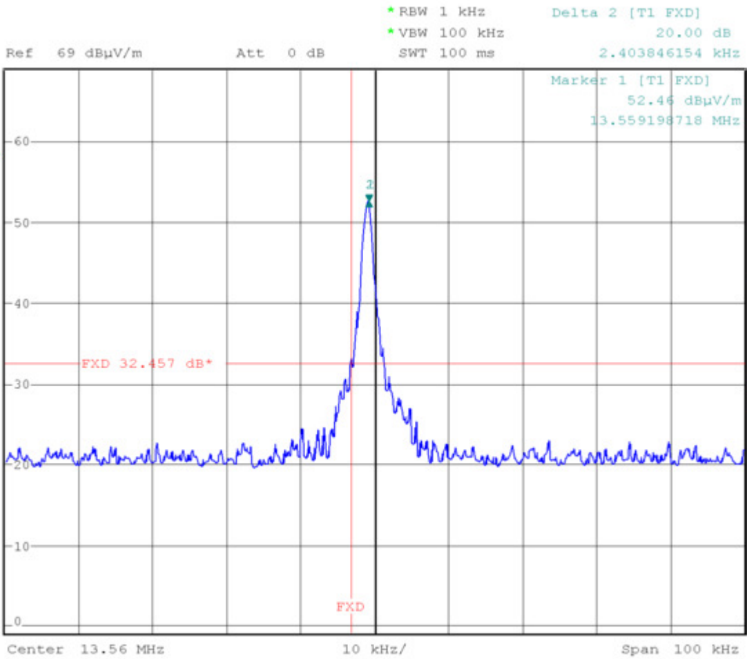
Picture 20: Occupied bandwidth lower value
