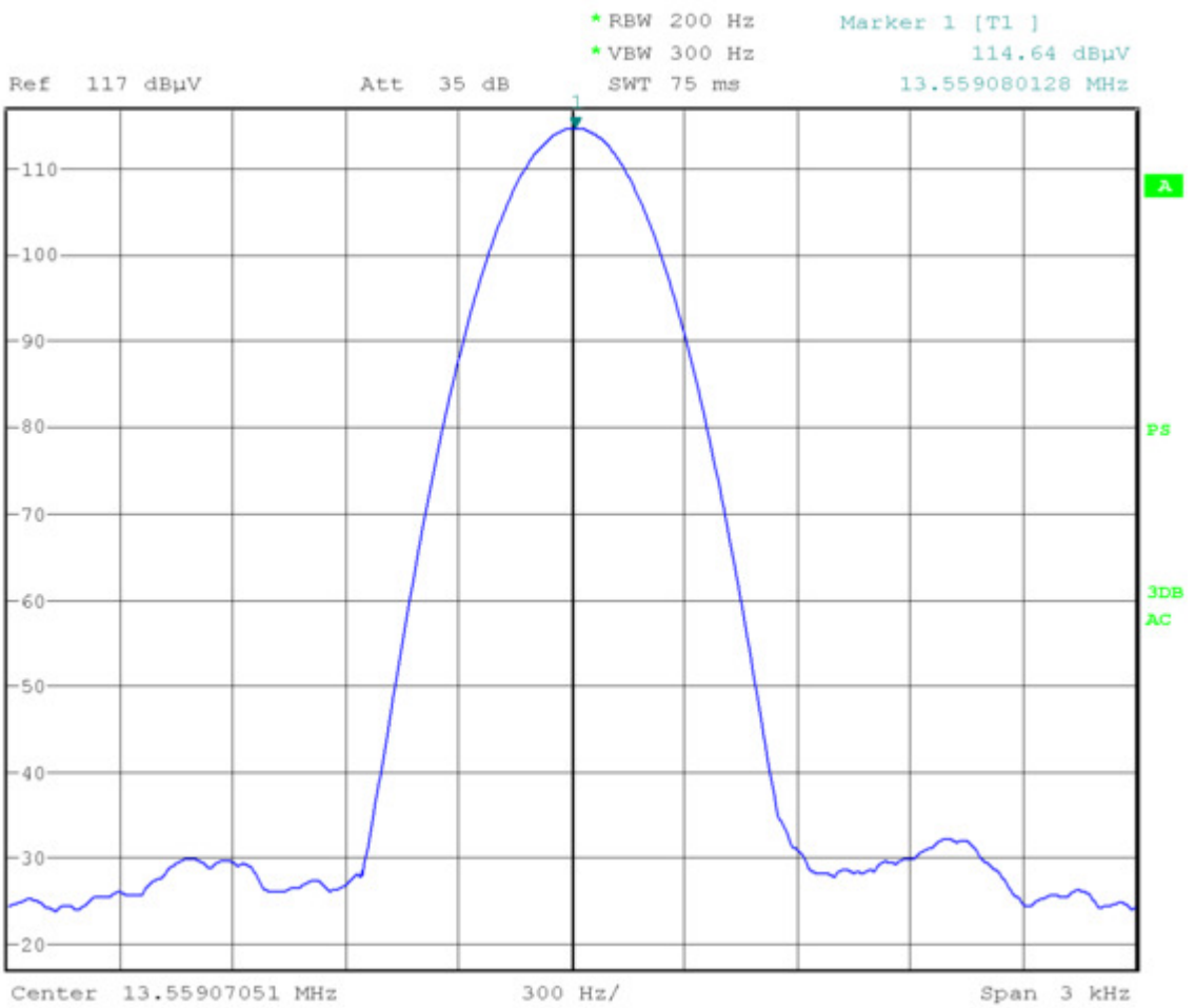
Picture 30: +50°C, 5 VDC
