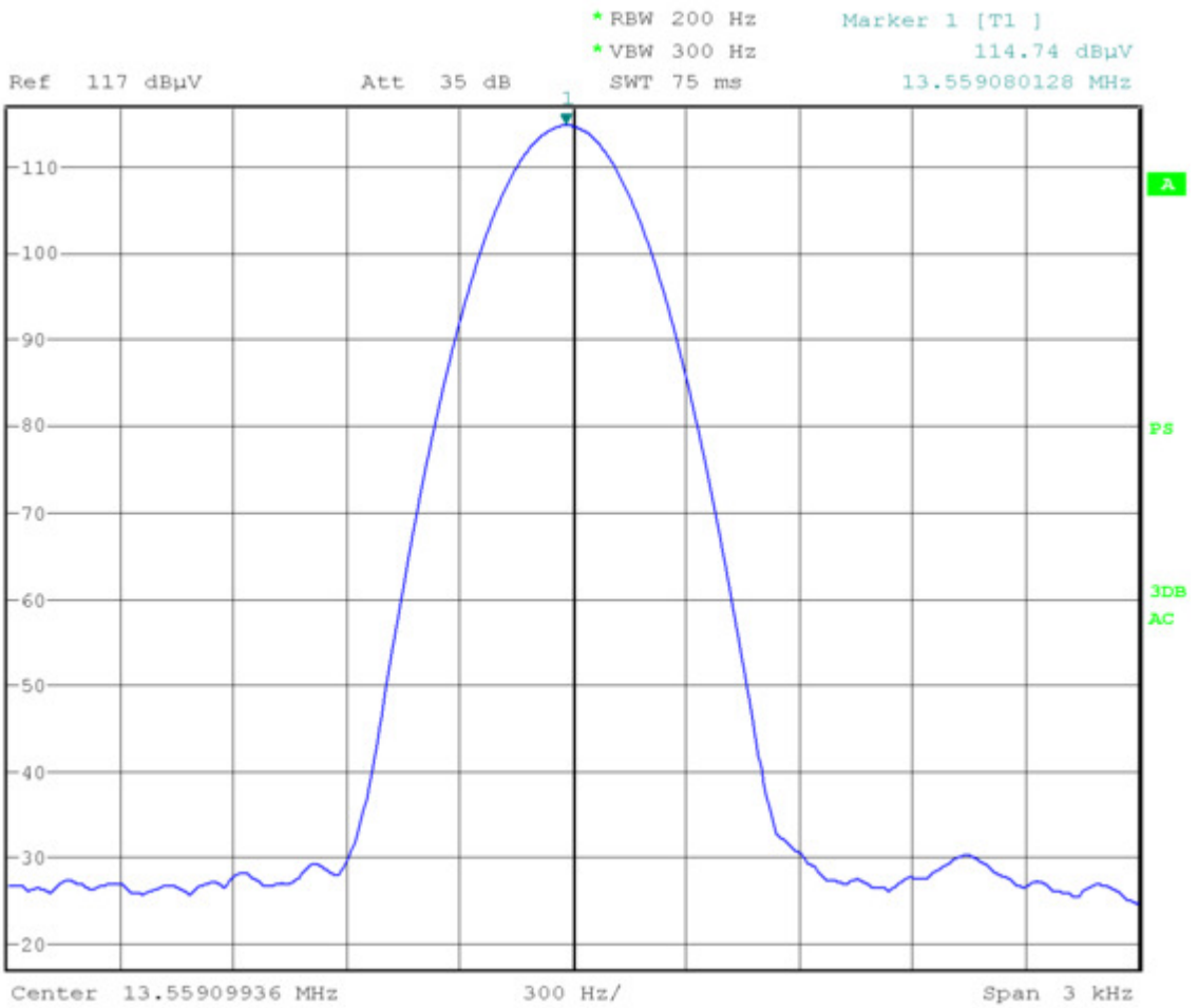
Picture 31: 20°C, 4.25 VDC
