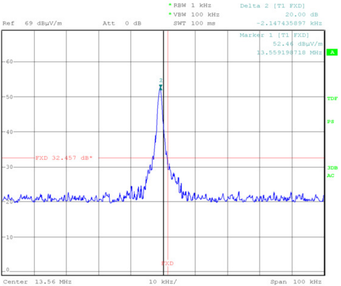
Picture 21: Occupied bandwidth upper value
