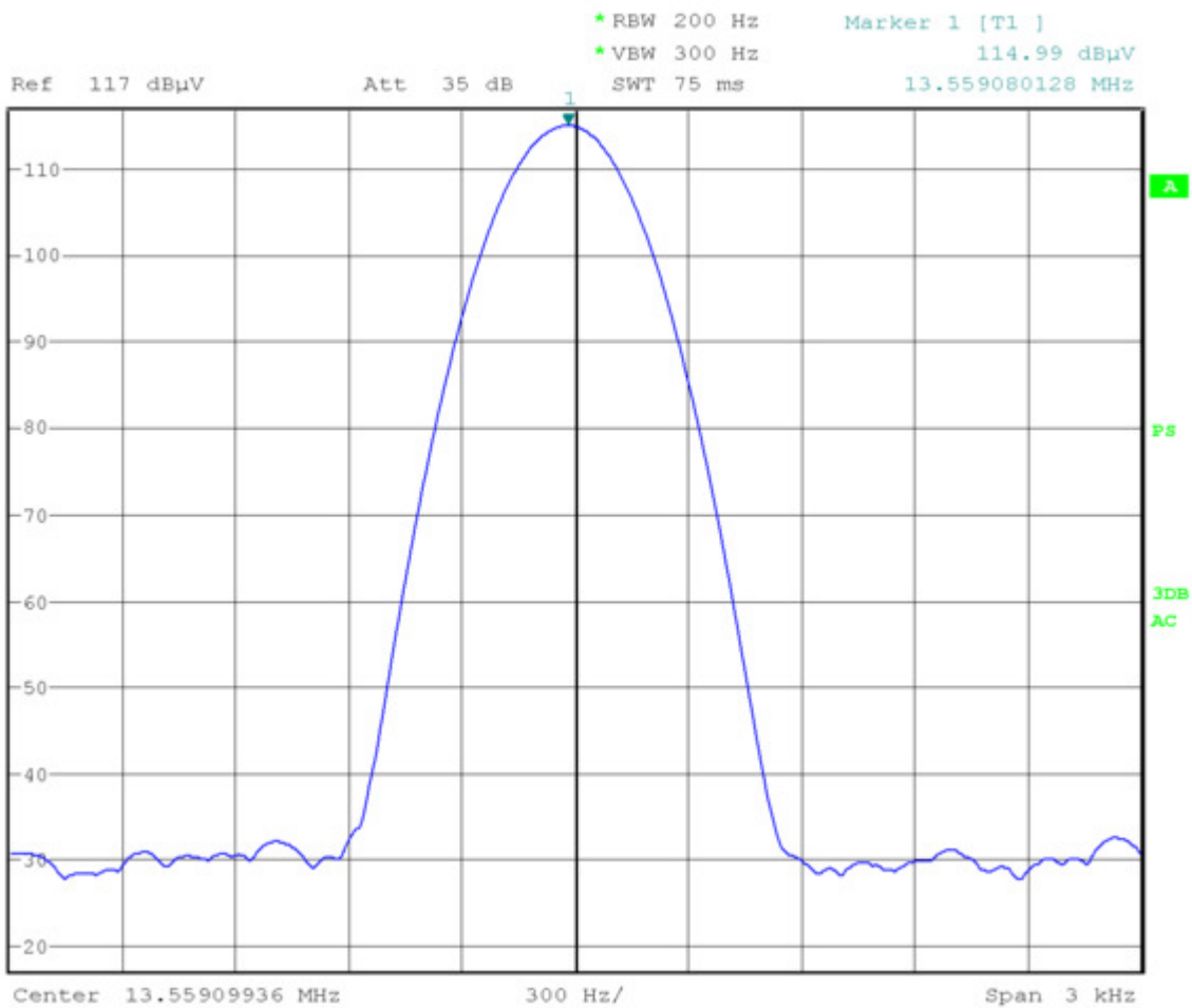
Picture 32: 20°C, 5.75 VDC
