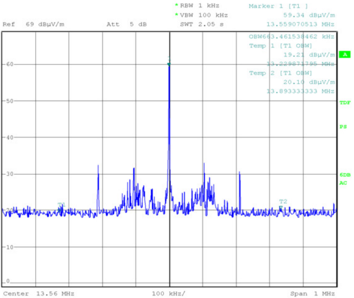
Picture 18: Occupied bandwidth 99%
